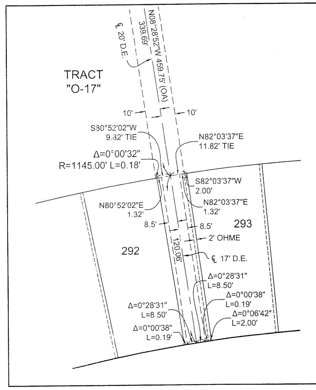
DETAIL "A" NOT TO SCALE
